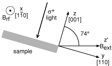
FIG. 1. The coordinate frame (x', y', z') is aligned to the external magnetic field B_{\text{ext}} and the (x, y, z) frame to the crystallographic axes of the sample. The incident laser light is parallel to the growth direction of the sample ( z ), and the radio frequency field B_{\text{rf}} is applied perpendicular to B_{\text{ext}} .
