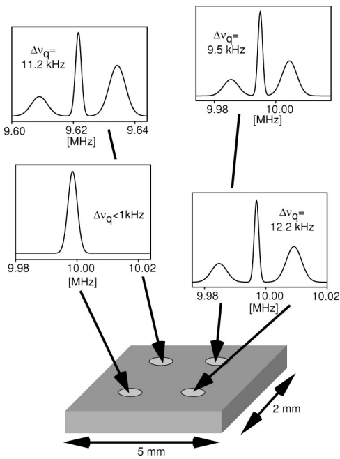
FIG. 4. Lateral change of quadrupole splitting. All spectra were recorded for a single quantum well of width 19.7 nm in an area smaller than 4 \text{ mm}^2 .
