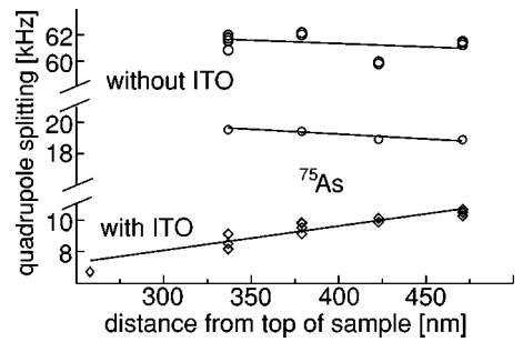
FIG. 5. Quadrupolar splittings of ^{75}\text{As} as a function of depth within the multiple quantum-well sample. The upper two sets were measured on a piece of the sample without an ITO layer on top, and the lower set was from a piece with an ITO layer on top. All three measurements were made at different positions on the sample.
