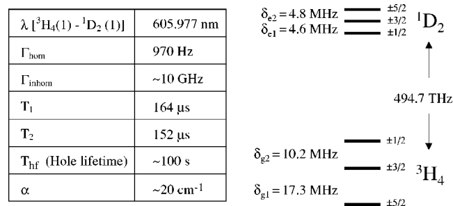
FIG. 4. Energy level diagram and relaxation data for the ^3\text{H}_4 - ^1\text{D}_2 transition of site I \text{Pr}^{3+} ions in \text{Y}_2\text{SiO}_5 . T_1 , T_2 , and \Gamma_{\text{hom}} are given according to Ref. 27.
