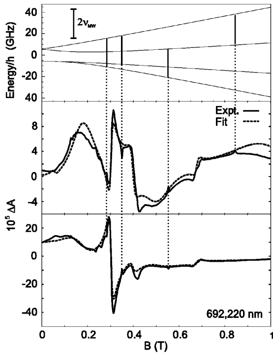
FIG. 13. Appearance of double quantum transition resonances demonstrated by spectra at 692.220 nm [absorption (top) and dispersion (bottom) phase].
