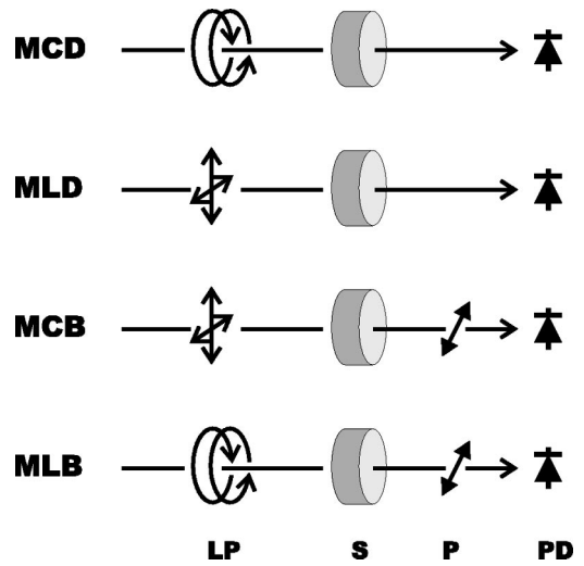
FIG. 5. Schematic optical setup for the detection of different magneto-optical effects (LP, polarization of the laser light; S, sample; P, polarizing filter 45°, PD, photo diode).
