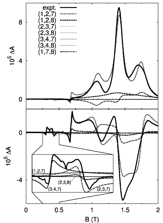
FIG. 9. Contributions of the different three-level subsystems to the absorption (top) and dispersion (bottom) phase of the spectrum at 692.081 nm. Solid line, measured spectrum, (k,l,m) , contribution of the subsystem of the three states \psi_k , \psi_l , and \psi_m to the fit. The inset shows the main contributions of the dispersion phase between 0.25 T and 0.5 T.
