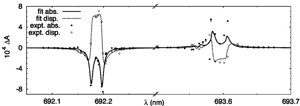
FIG. 8. Wavelength dependence of the magnetic resonance at 0.3 T. Experimental amplitudes are shown as circles, fits as lines. (solid line, circle: absorption; dotted line, open circle: dispersion).
