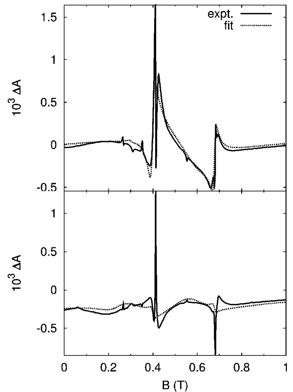
FIG. 14. Narrow lines at the EPR resonances at 693.578 nm [absorption (top) and dispersion (bottom) phase].
