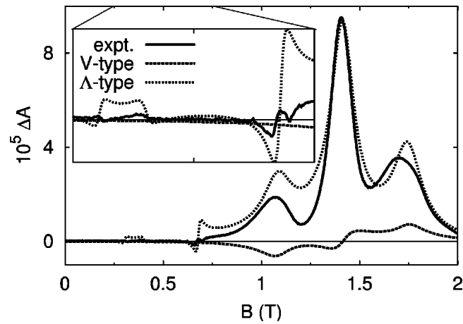
FIG. 11. Contributions of V- and \Lambda -type configurations to the absorption phase of the spectrum at 692.081 nm. The inset depicts the detail between 0.25 T and 0.75 T.
