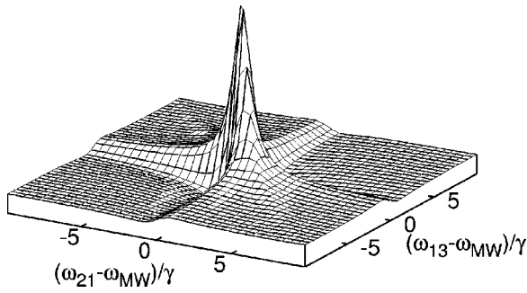
FIG. 3. Microwave and laser frequency dependence of \Lambda_{123}(\omega_L, \omega_{MW}) in arbitrary units (with \gamma = \gamma_{12} = \gamma_{13} = \gamma_{23} and equal population differences). Only the real part is shown.
