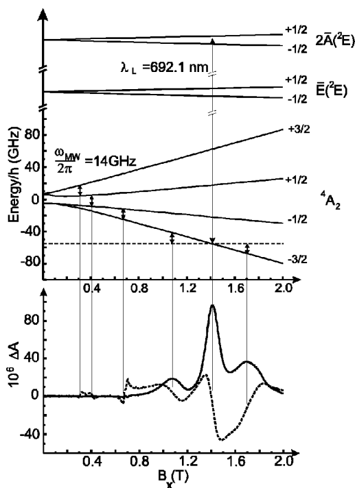
FIG. 1. Energy diagram and Raman-heterodyne spectrum of ruby, detected with a laser tuned close to the R_2 transition (solid line, absorption phase; broken line, dispersion phase). The absorption difference \Delta A refers to the difference between the absorption of left and right circularly polarized light. The arrows indicate the transitions that give rise to the different resonance lines.
