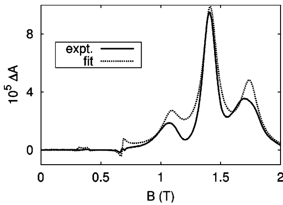
FIG. 7. An example of a fitted experimental spectrum at 692.081 nm (simulated spectrum, dashed line; experimental spectrum, straight line).
