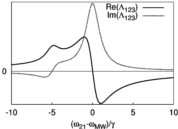
FIG. 4. Microwave frequency dependence of \Lambda_{123} at a normalized optical detuning (\omega_{13} - \omega_L)/\gamma = 5 . The resonance at \omega_{21} - \omega_{MW}/\gamma = -5 is the Raman resonance running diagonally through Fig. 3. The resonance at \omega_{21} = 0 is the EPR transition.
