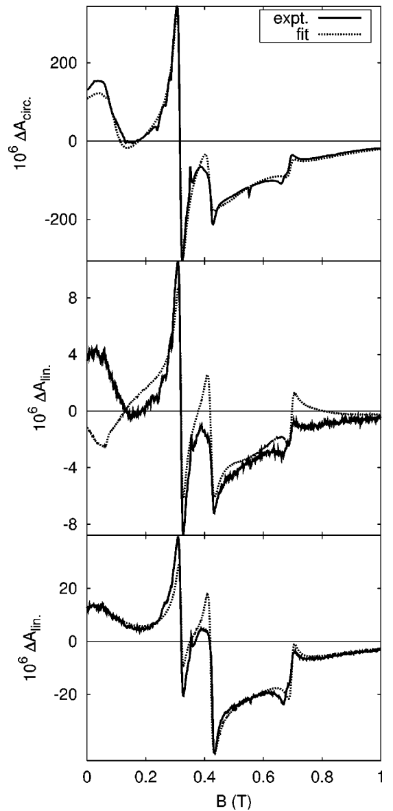
FIG. 12. Comparison of spectra (dispersion phases at 692.20 nm) taken with MCD, MLD, and MCB configurations.
