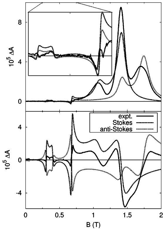
FIG. 10. Contributions of the Stokes and anti-Stokes-Raman waves to the absorption (top) and dispersion (bottom) phases of the spectrum at 692.081 nm. The inset shows the main contributions of the absorption phase between 0.25 T and 0.75 T.
