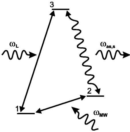
FIG. 2. Coherent Raman process in a three-level system.
