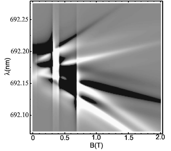
FIG. 6. Density plot of the absorption component of the Raman-heterodyne signal as a function of the magnetic-field strength and the laser frequency in the vicinity of the R_2 line.
